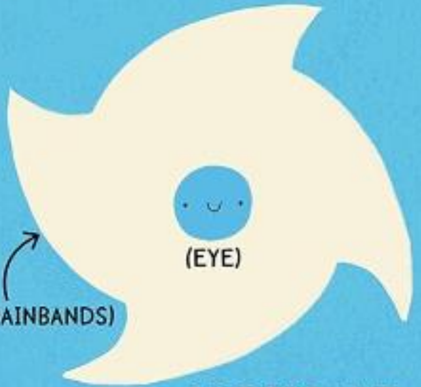
HURRICANE
