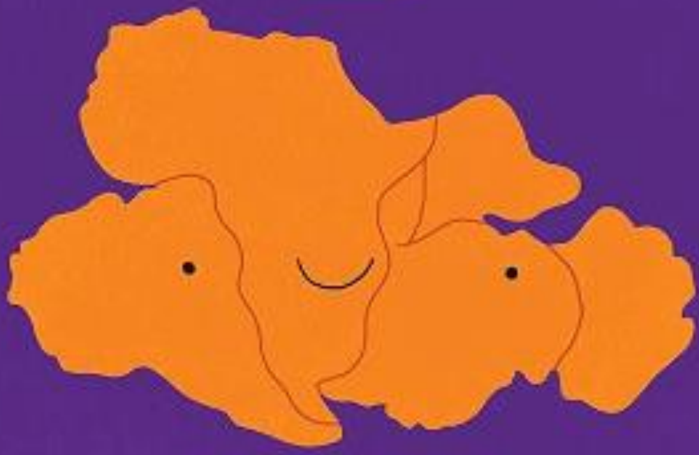
GONDWANA (SUPERCONTINENT)
